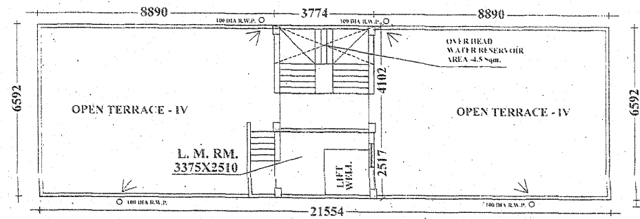
ROOF PLAN SCALE - 1:100
