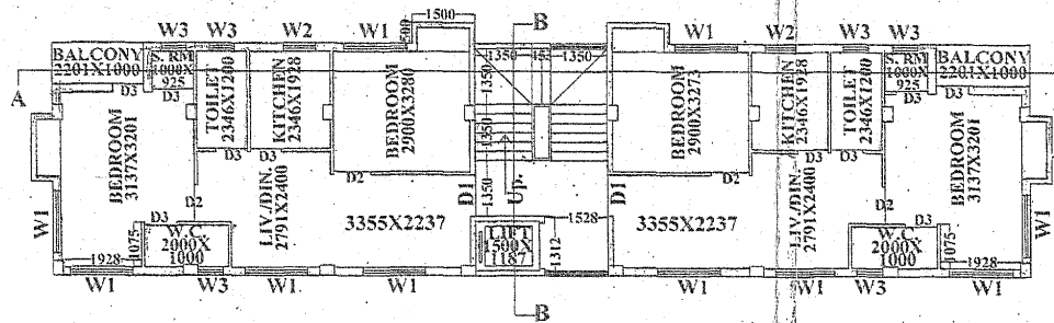
TYPICAL FLOOR PLAN (1ST, 2ND, 3RD AND 4TH FLOOR SEMILAR) BLOCK - B
