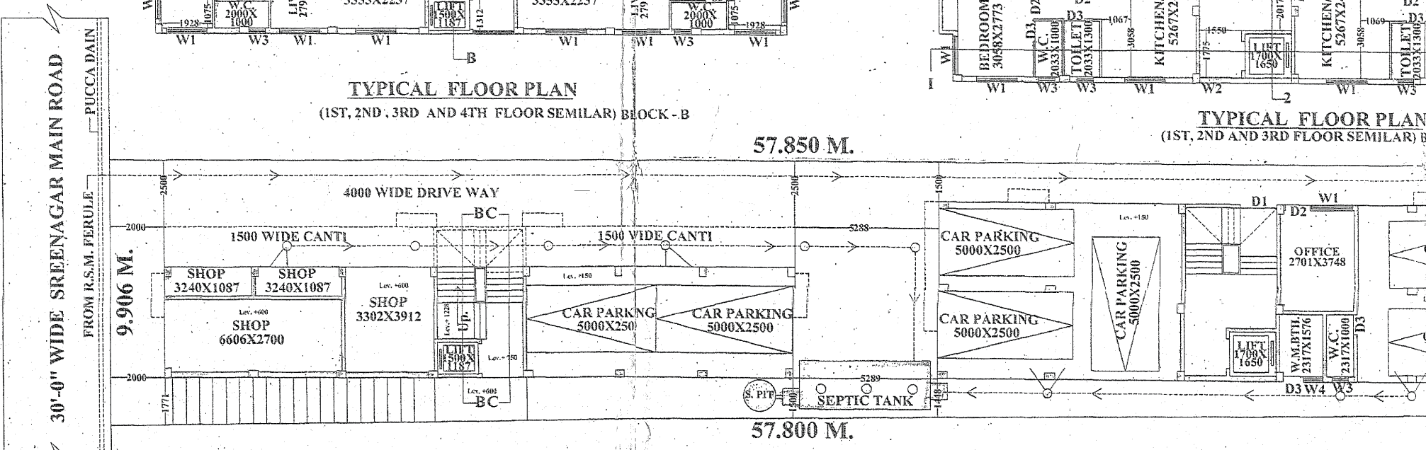
GROUND FLOOR PLAN SCALE - 1:100
