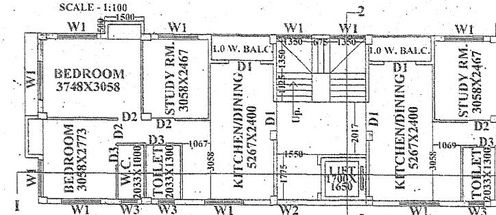
TYPICAL FLOOR PLAN (1ST, 2ND AND 3RD FLOOR SEMILAR) BLOCK - C
