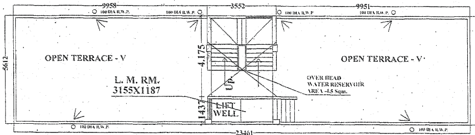
ROOF PLAN SCALE - 1:100
